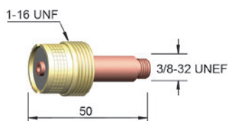
Large Long Gas Lens 大长气筛
